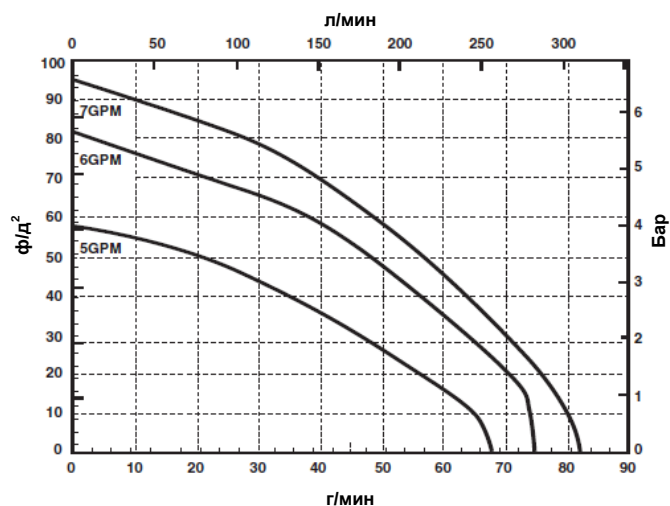
9303P-NM2C
