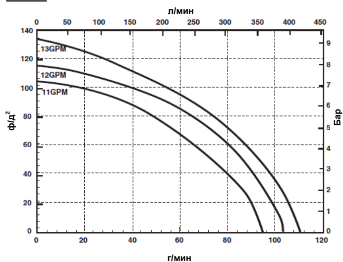
9303 9303P-NM1C
