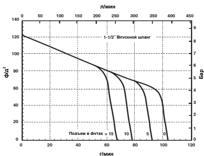
9303C-HM2C & 9303S-HM2C
