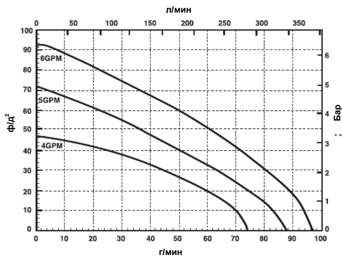
9303C-HM2C & 9303S-HM2C
